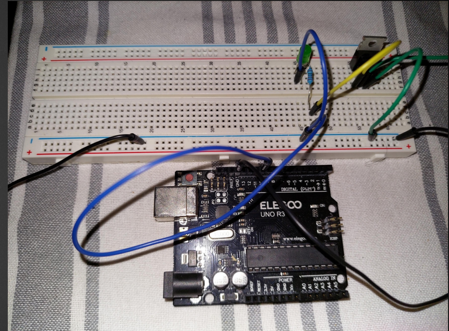
Figure 6: GA HDRM Team's Final Circuit
