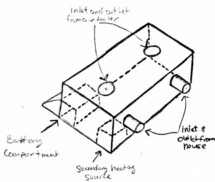
Figure 18: Vertically Heated Box with Heat Circulation, Control System and Secondary Heat Source (Inside Concept View)
