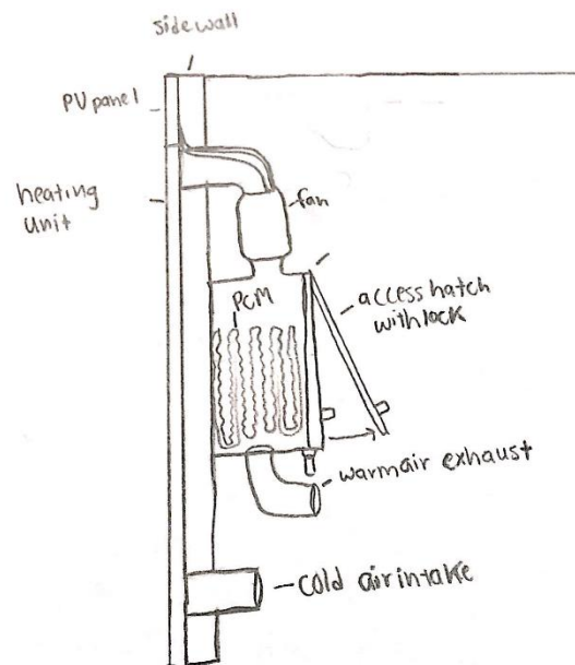
Figure 10: Wall-Mounted Constant Heating Device
