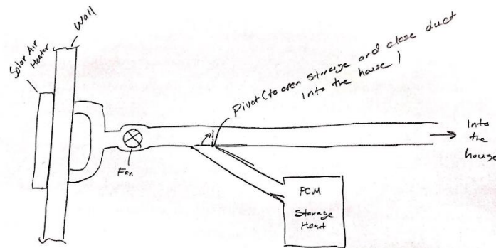
Figure 11: Switch-Based Ducted Heating Storage
