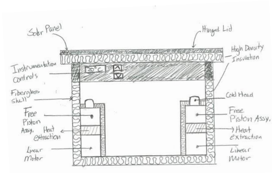
Figure 18: Solar powered Ice-Chest.
