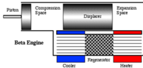
Figure 4: Schematic of Beta type Stirling engine [14]
