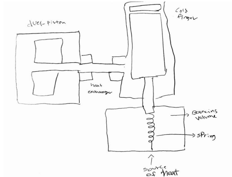
Figure 19: Dual piston
