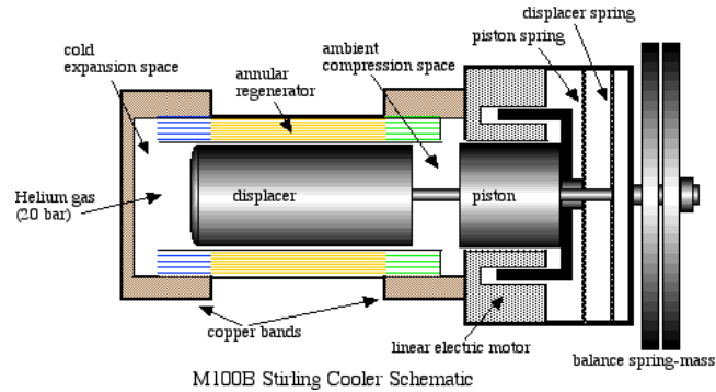
Figure 6: Schematic of Free Piston cooler [1].
