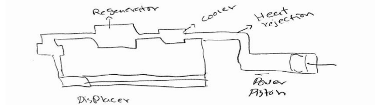
Figure 20: Inline regenerative cryocooler
