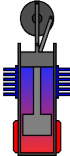
Figure 3: Beta type Stirling engine [14]
