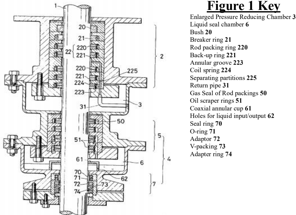
Figure 11: Piston Rod Sealing arrangement from Eisuke Sugahara [20]
