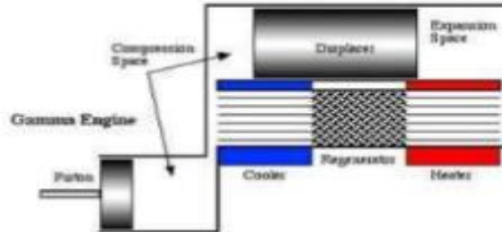
Figure 5: Gamma engine existing design 3 [5]
