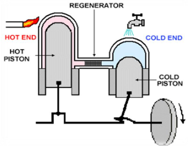
Figure 4: Alpha engine existing design 1 [1]
