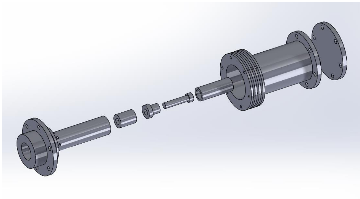
Figure 28 Updated assembly of cold head, heat exchanger, and inner piston/displacer.
