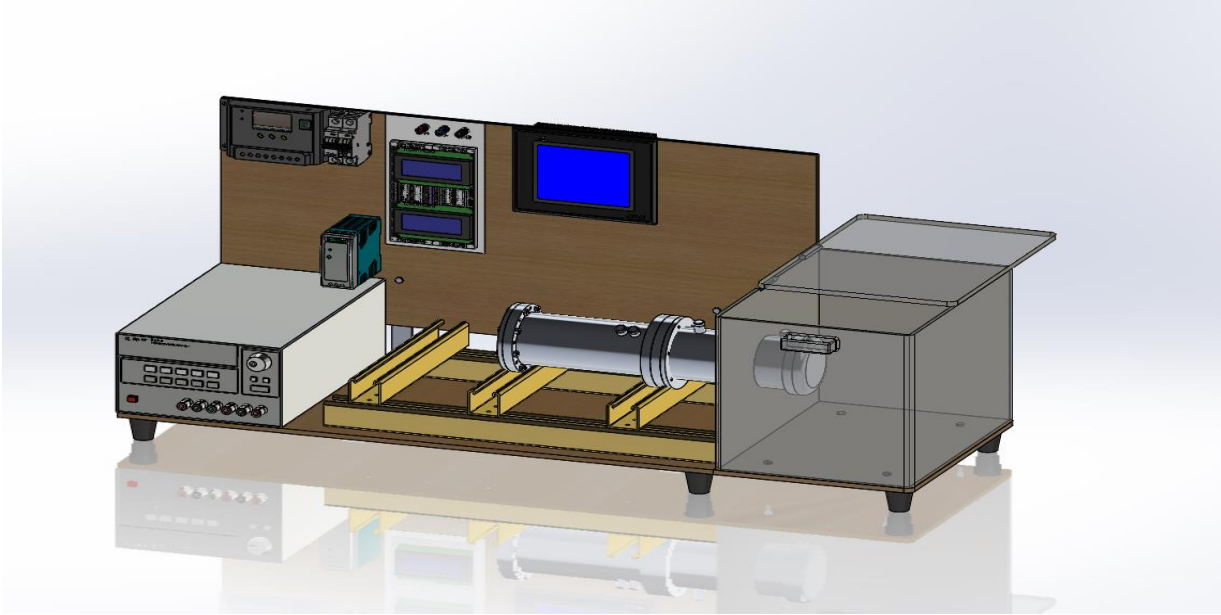
Figure 27: New Assembly CAD
