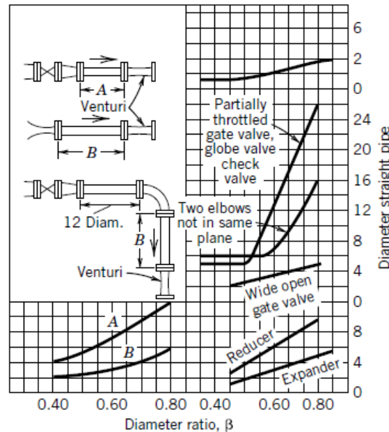
Figure 7.2.5b: Venturi flowmeter diameter ratio.
