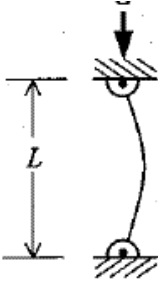
Figure 19 Buckling load on a beam [3]
