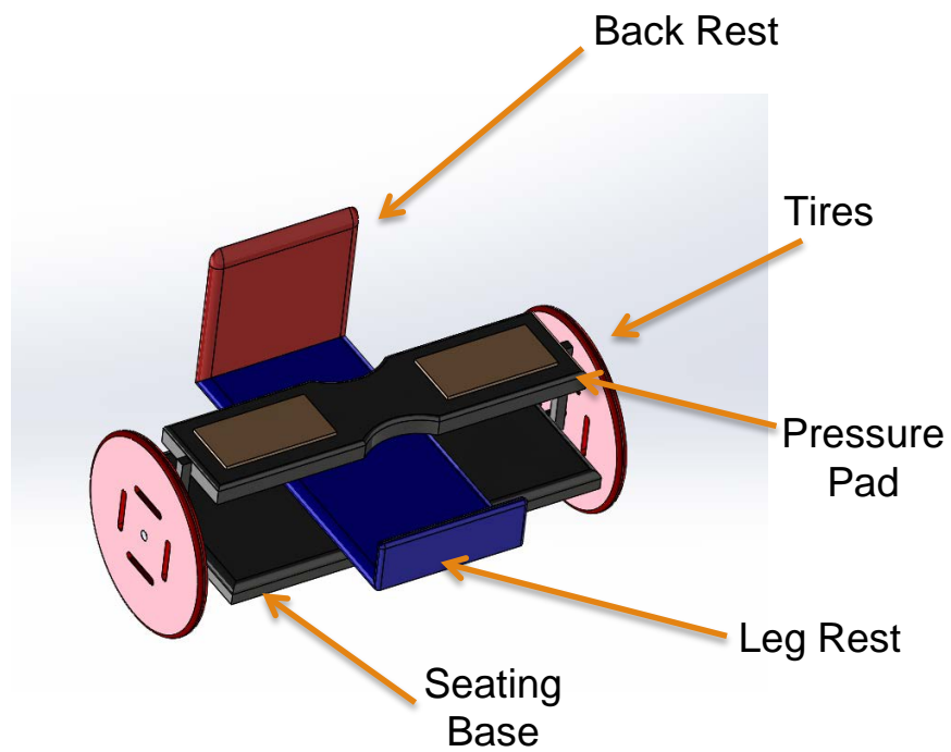
Figure 2: Capstone part 1 final PPT CAD design
