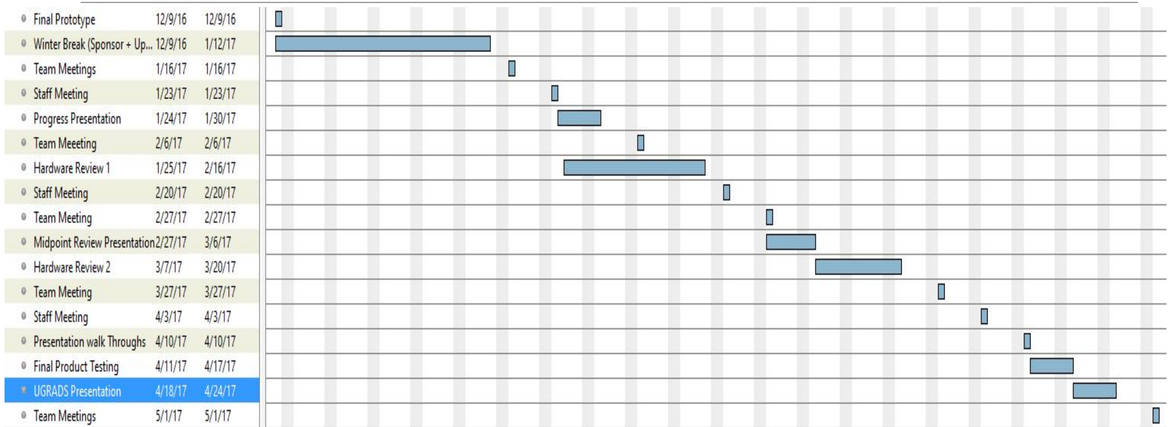
Figure 7: Gantt Chart
