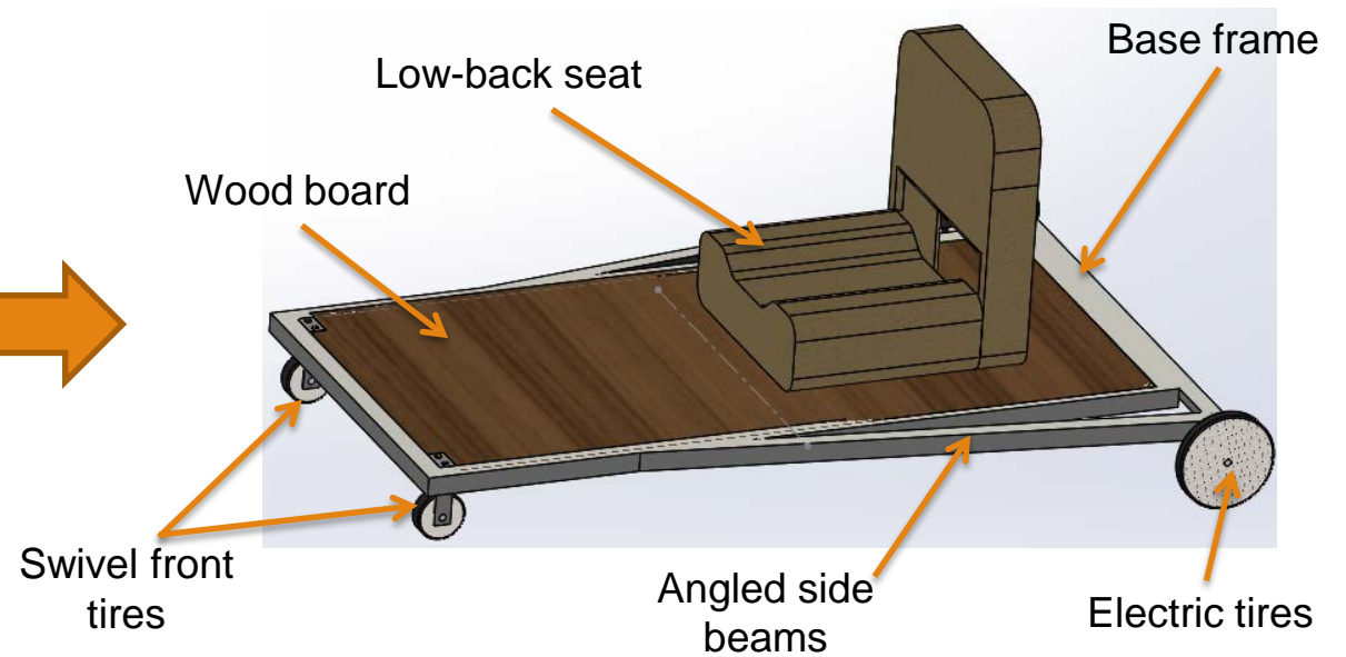
Figure 3: Current CAD design
