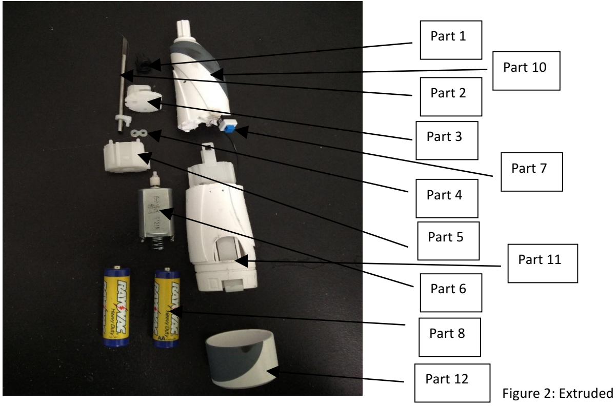
Figure 2: Picture of electric toothbrush
