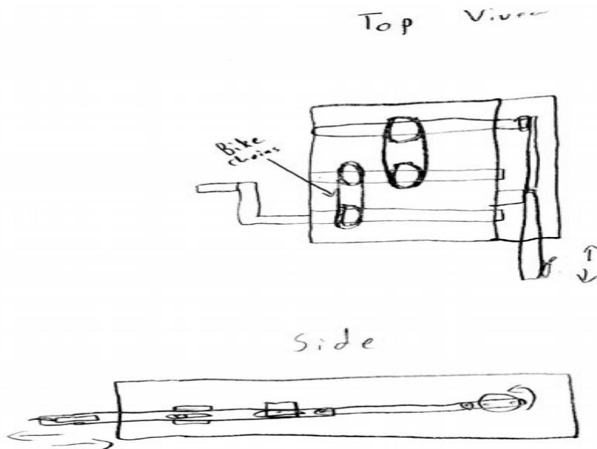
Figure 8: Chain design
