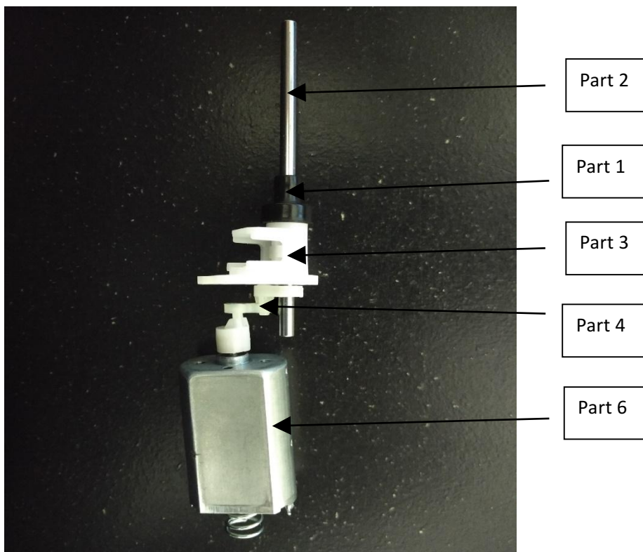
Figure 4: Attachment design
