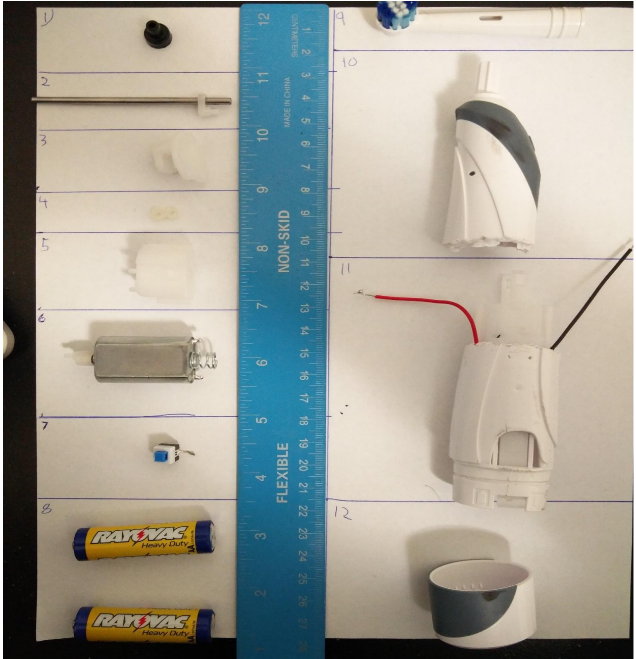
Figure 3: Electric Toothbrush parts
