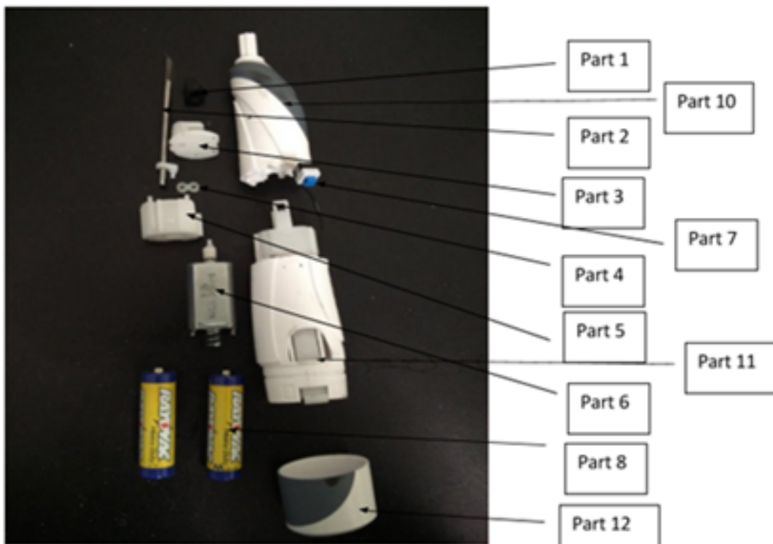
Figure 19: Toothbrush assembly
