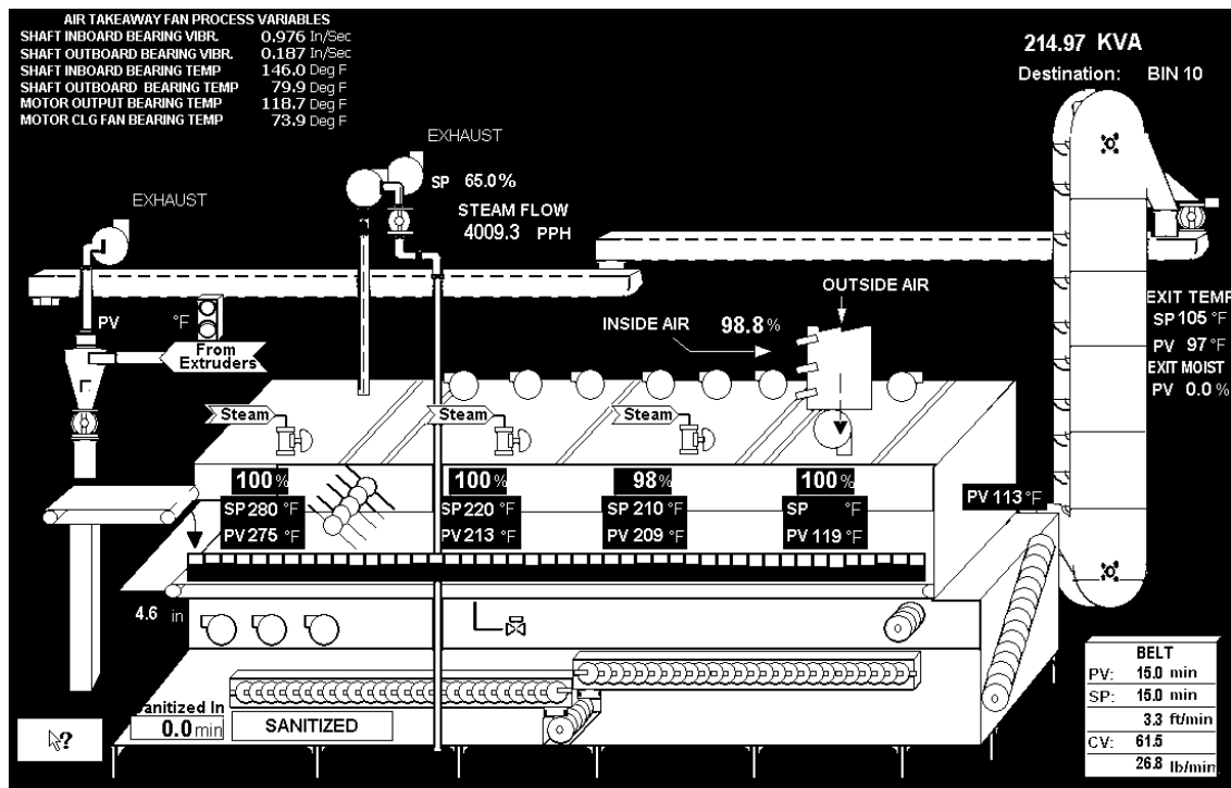
Figure 5 - Dryer 3 Source: Nestle Purina Process Monitoring System
