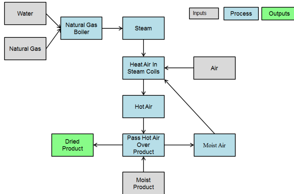
Figure 3 – Function Diagram
