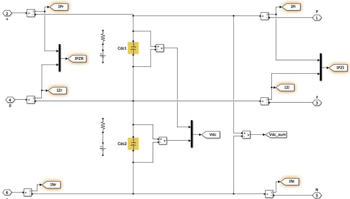
Fig. 5. Simulation (DC-Link) NPC Converter for Wind Turbines.
