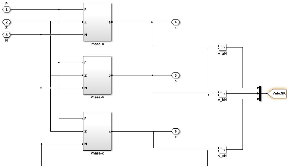
Fig. 6. Simulation (3L Inverter) NPC Converter for Wind Turbines.
