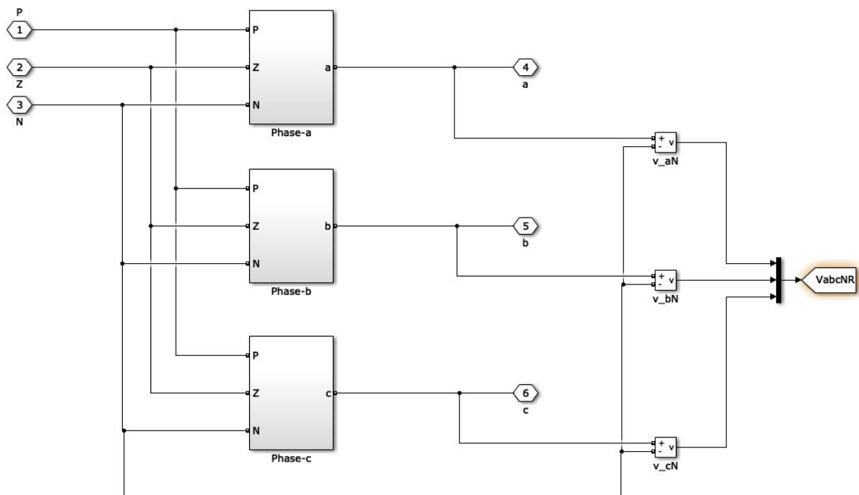
Fig. 4. Simulation (3L Rectifier) NPC Converter for Wind Turbines.
