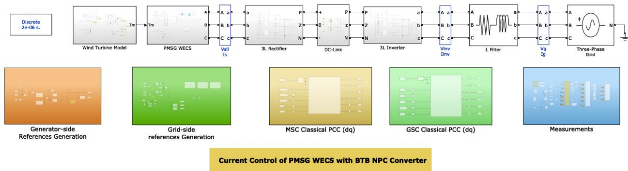
Fig. 1. Simulation NPC Converter for Wind Turbines.
