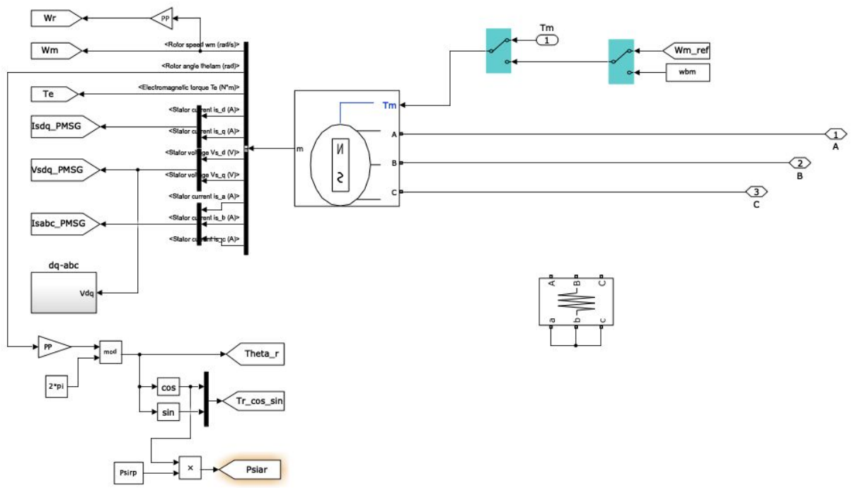
Fig. 3. Simulation (Motor) NPC Converter for Wind Turbines.
