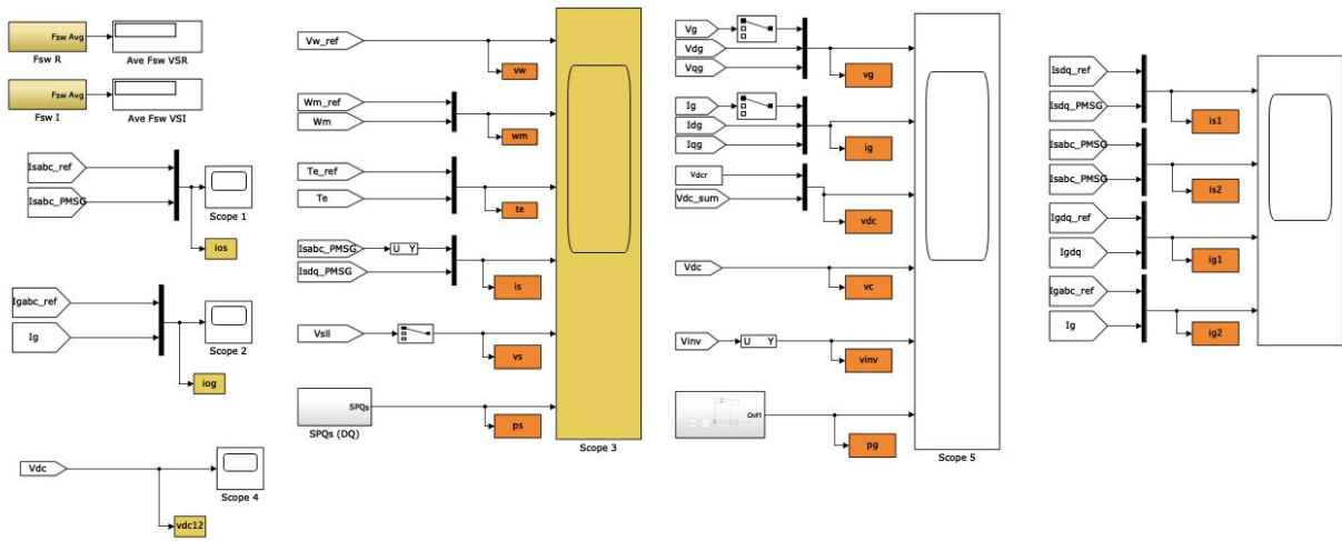
Fig. 7. Simulation (3L Inverter) NPC Converter for Wind Turbines.
