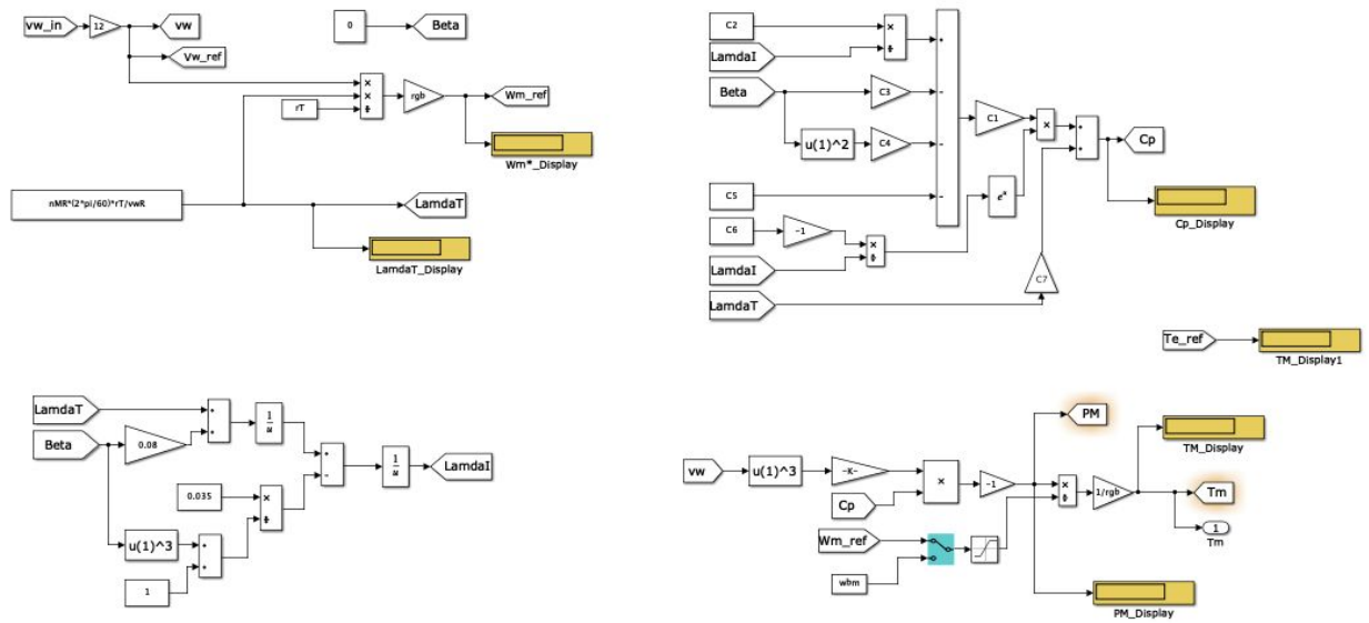
Fig. 2. Simulation (wind) NPC Converter for Wind Turbines.
