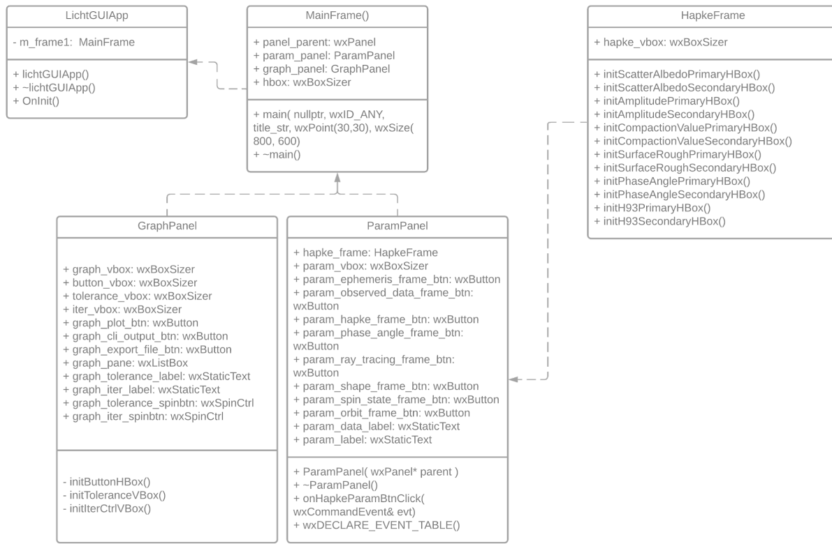
Figure 5. UML diagram of the Licht GUI app prototype
