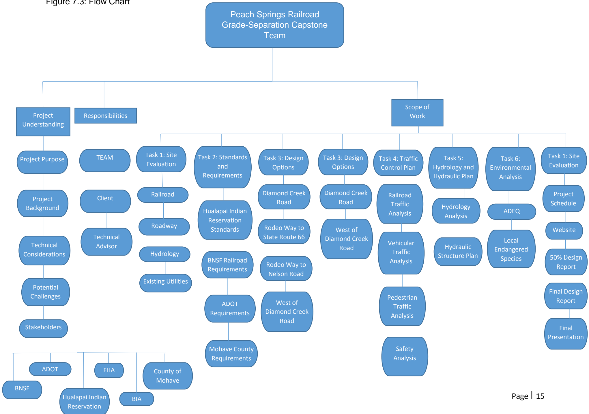
Figure 7.3: Flow Chart
